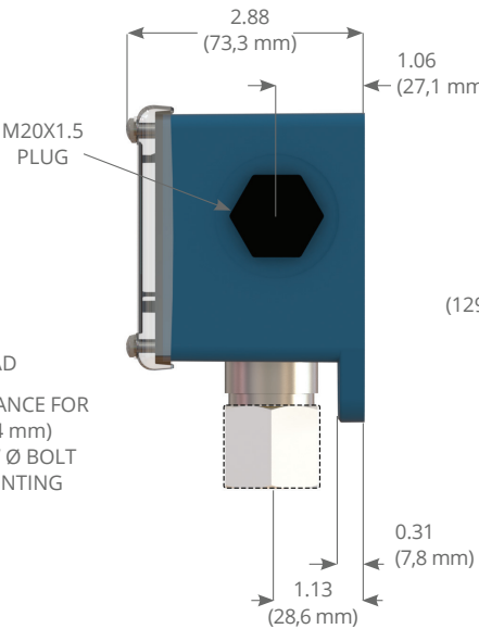
Model 1GSWLL Enclosure and Sensor Details
