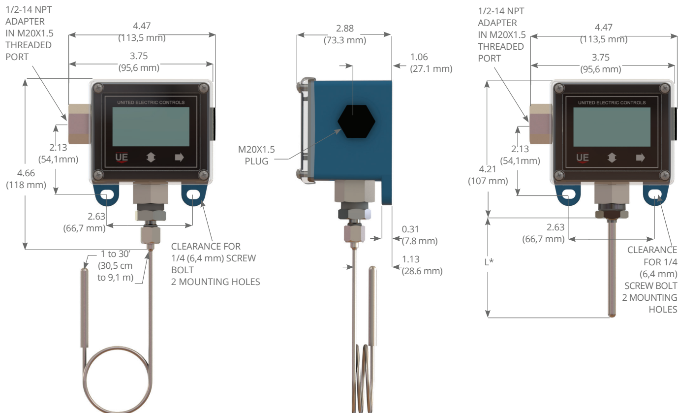
Model 1GSWLL Enclosure and Sensor Details
